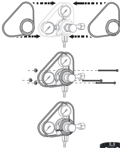
JE-742GCN INSTALLATION GUIDE
